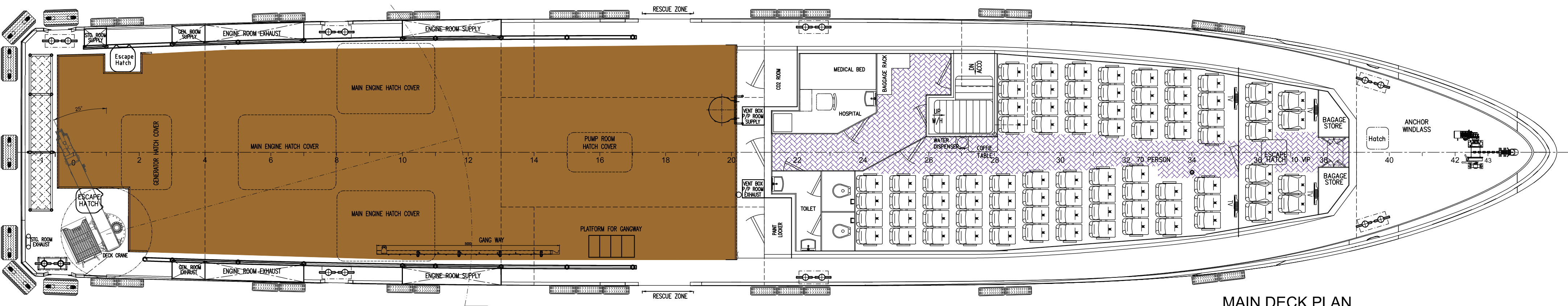
MAIN DECK PLAN
