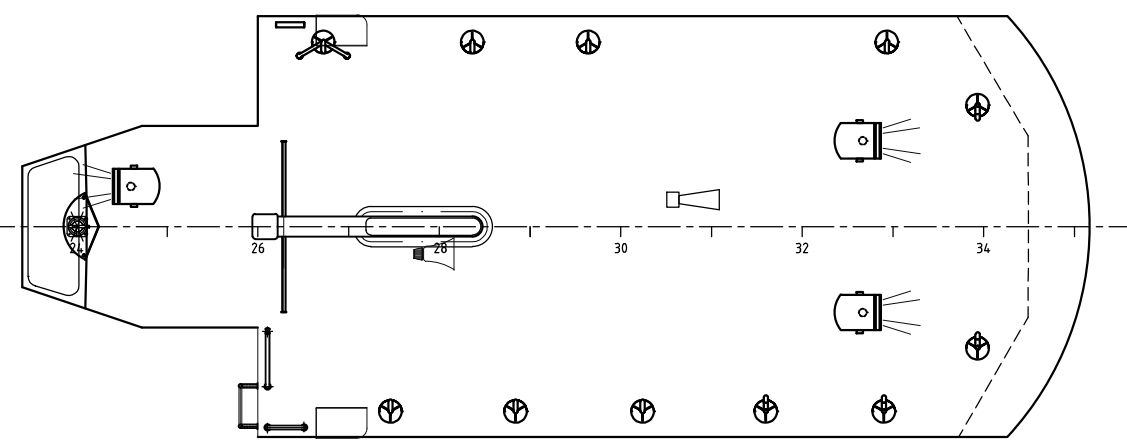
WHEEL HOUSE TOP DECK
